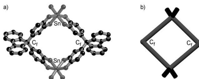
Figure 1. a) The chiral [L 2 {Sn(OH) 2 }] 2 4- macrocycle. b) Schematic representation of the macrocycle in which the corners represent the tetrahedral fluorene carbon atoms, C f , and the dihydroxytin centers.
